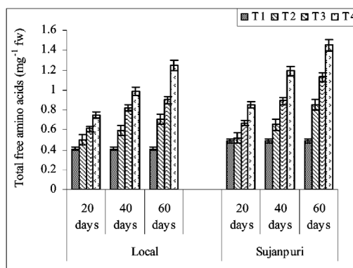
Figure 4. Effect of different concentration of NaHCO 3 on Total free amino acids. Values are significantly different P < 0.05 from control (DMRT). Values are means \pm S.E (n = 5).
