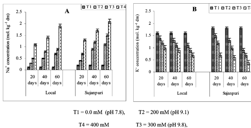
Figure 6. Effect of different concentration of \text{NaHCO}_3 on (A) \text{Na}^+ concentration ( \text{mol. Kg}^{-1} DM) and (B) \text{K}^+ concentration ( \text{mol. Kg}^{-1} DM). Values are significantly different p < 0.05 from control (DMRT). Values are means \pm S.E (n = 5).
