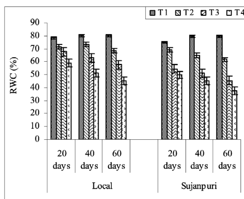
Figure 3. Effect of different concentration of NaHCO 3 on Relative water content (%). Values are significantly different P < 0.05 from control (DMRT). Values are means \pm S.E (n=5).
